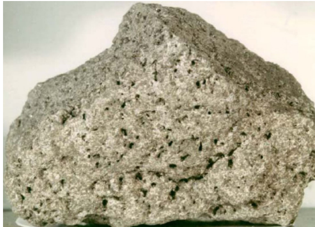
Figure 9.10 Rock from a Lunar Mare. In this sample of basalt from the mare surface, you can see the holes left by gas bubbles, which are characteristic of rock formed from lava. All lunar rocks are chemically distinct from terrestrial rocks, a fact that has allowed scientists to identify a few lunar samples among the thousands of meteorites that reach Earth. (credit: modification of work by NASA)
